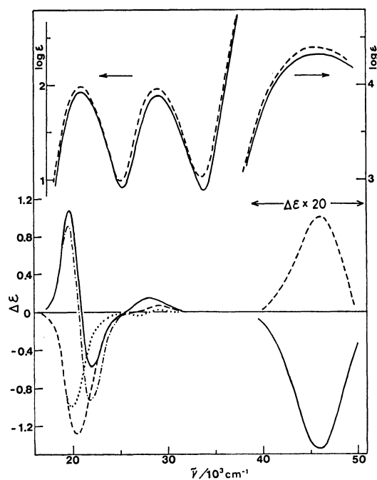
Fig. 5. Absorption and CD spectra of A -[Co(en) 2 ( R -mtmd)] 3+ (M-I-1) in water (—) and in 0.2 mol/dm 3 Na 2 SO 4 (---), and A -[Co(en) 2 ( R -mtmd)] 3+ (M-II-2) in water (—) and in 0.2 mol/dm 3 Na 2 SO 4 (---).
