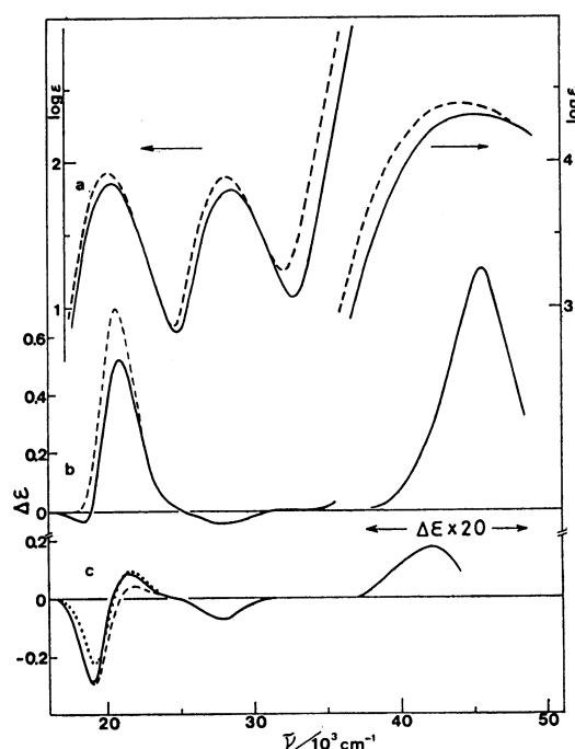
Fig. 8. a. Absorption spectra of cis - \Delta -[Co(NH _3 ) _2 (tmd) _2 ] ^{3+} (—) and cis - \Delta -[Co(NH _3 ) _2 {(—)-dmtmd} _2 ] ^{3+} (-----) in water. b. CD spectra of cis - \Delta -[Co(NH _3 ) _2 (tmd) _2 ] ^{3+} in water (—) and in 0.2 mol/dm ^3 Na _2 SO _4 (-----). c. CD spectra of cis - \Delta -[Co(NH _3 ) _2 {(—)-dmtmd} _2 ] ^{3+} in water (—) and in 0.2 mol/dm ^3 Na _2 SO _4 (-----), and the calculate dCD curve, 2 \times \Delta\epsilon [Co(NH _3 ) _4 {(—)-dmtmd} _2 ] ^{3+} + \Delta\epsilon ( cis - \Delta -[Co(NH _3 ) _2 (tmd) _2 ] ^{3+} ) (.....).
